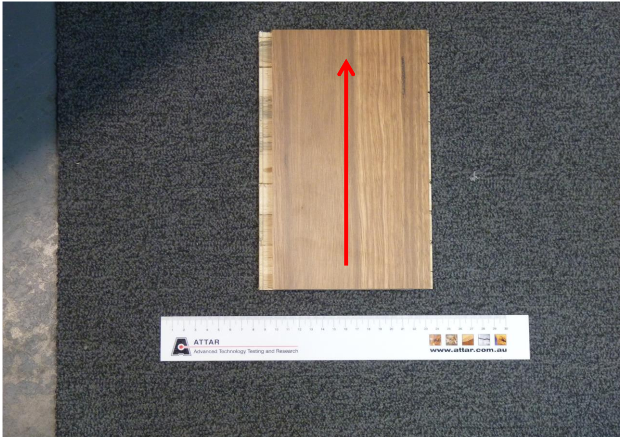
Figure 1: AU Naturale Reclaim Australian Species Engineered Timber Veneer Pre Finished Matt Coating Arrow indicates direction of testing
